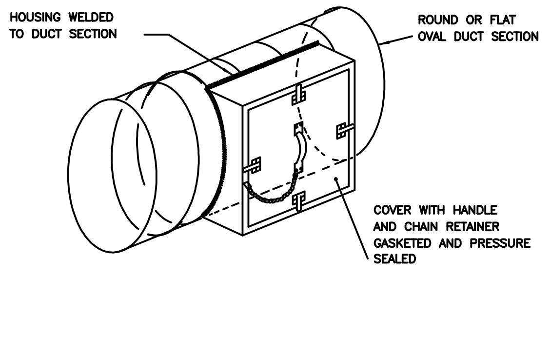
3 ACCESS PANEL FOR OVAL/ROUND DUCT M4.3 NO SCALE
