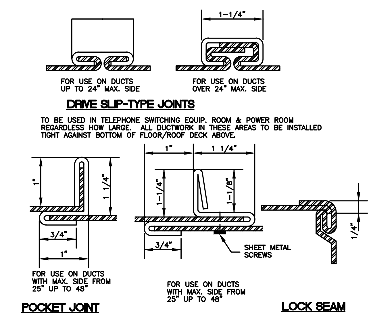
7 DUCT JOINTS AND SEAMS DETAIL M4.3 NO SCALE
