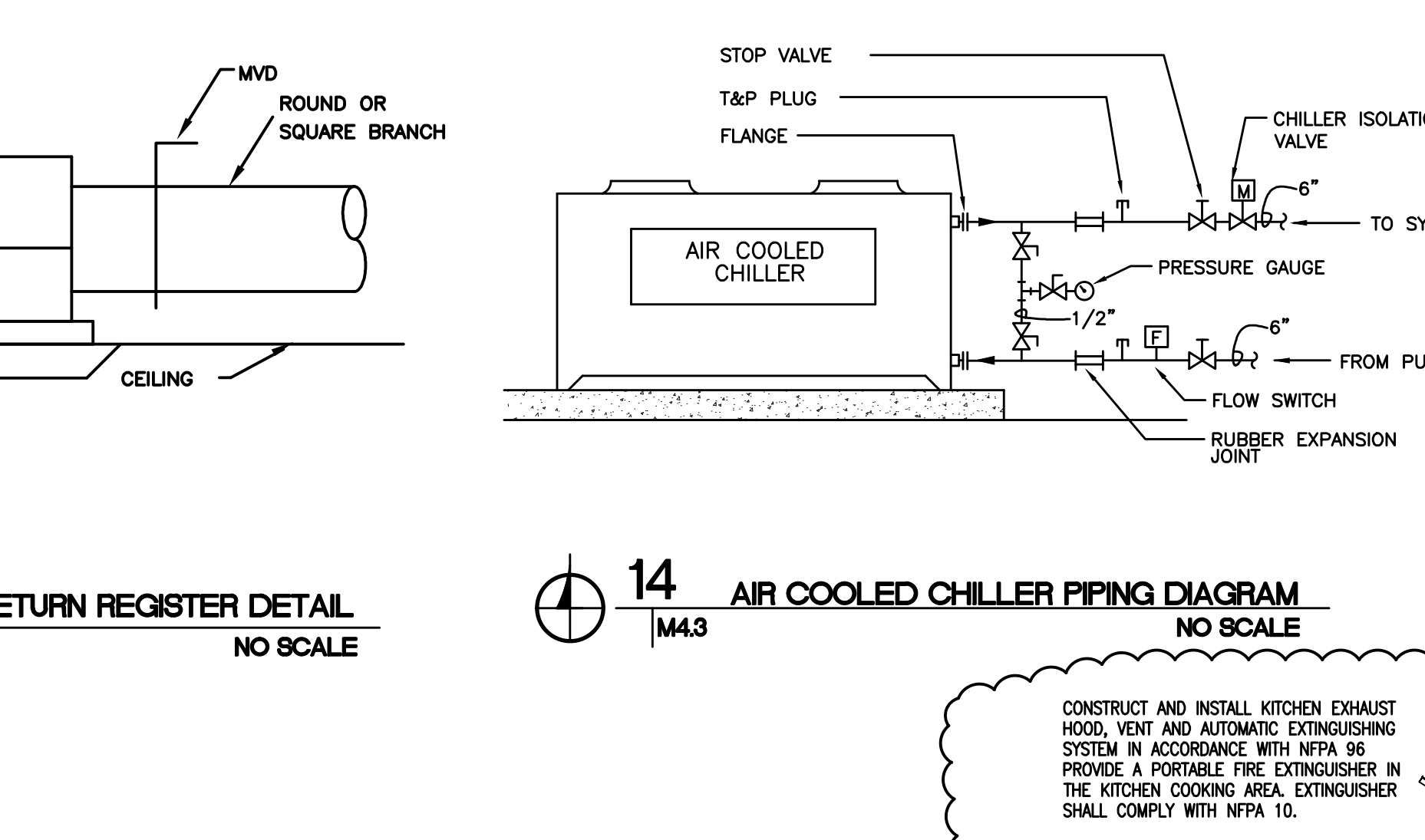
14 AIR COOLED CHILLER PIPING DIAGRAM M4.3 NO SCALE
