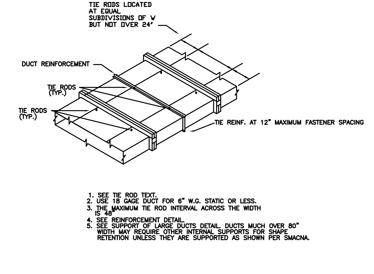
8 WIDE DUCT TIE ROD - INTERNAL SUPPORT DETAIL (DUCTS GREATER THAN 48" WIDE) M4.3 NO SCALE
