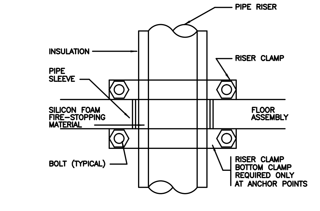
1 PIPE SUPPORT/ANCHOR THRU FLOOR SLAB M4.3 NO SCALE
