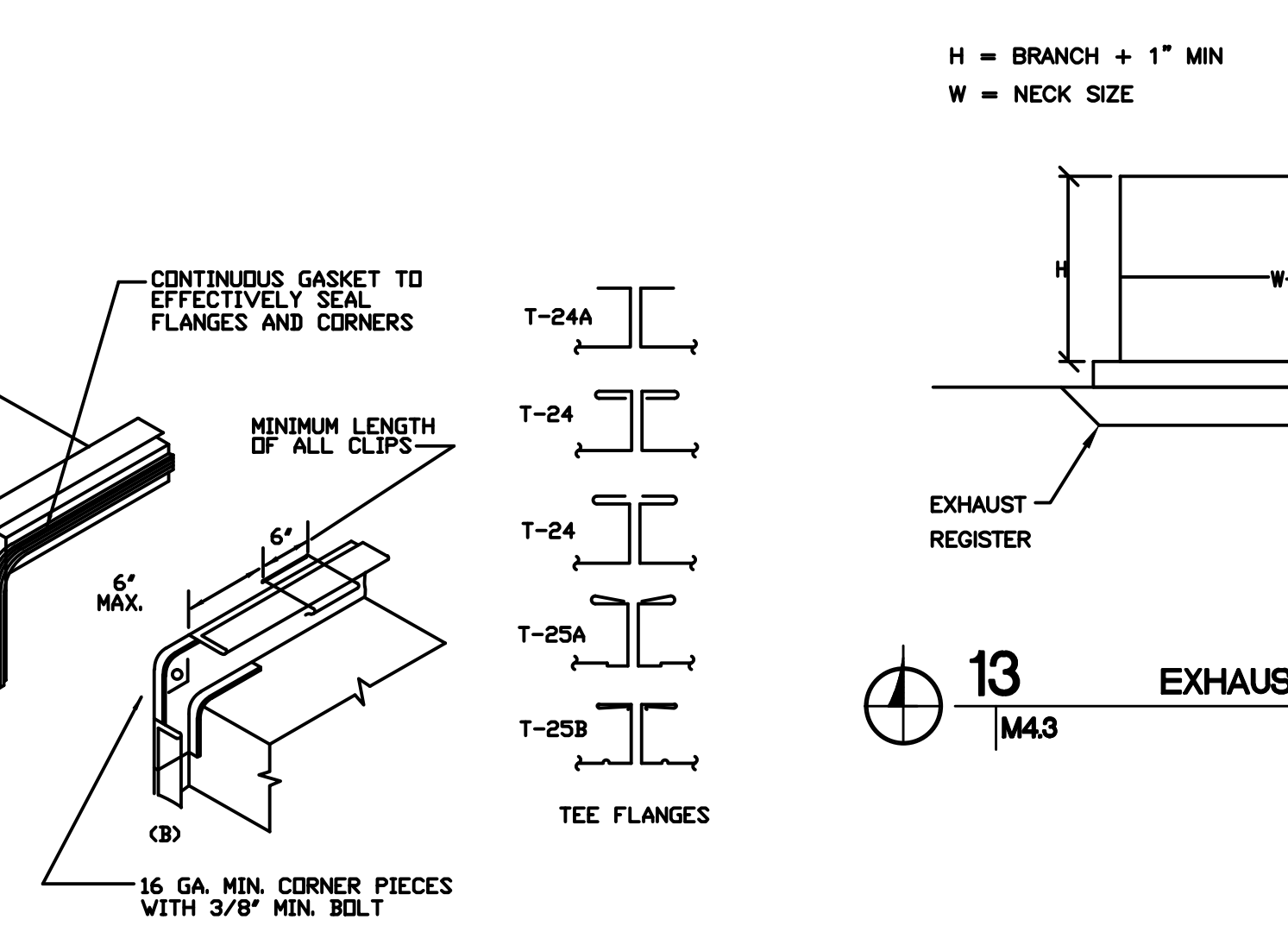
13 EXHAUST/RETURN REGISTER DETAIL M4.3 NO SCALE
