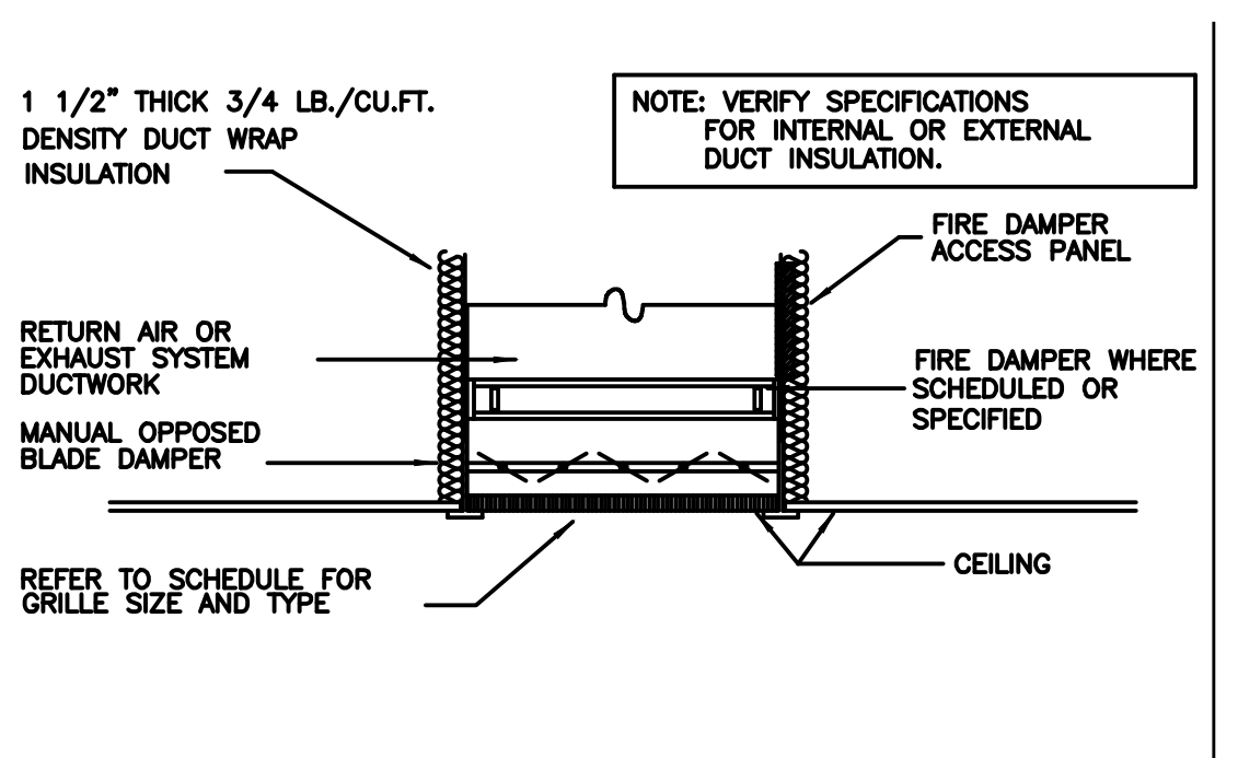
6 EXHAUST/RETURN GRILLE DETAIL M4.3 NO SCALE
