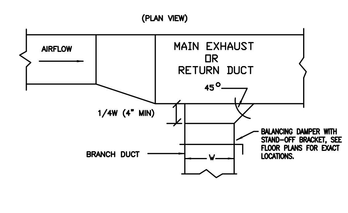
2 EXHAUST/RETURN BRANCH DUCT DETAIL M4.3 NO SCALE
