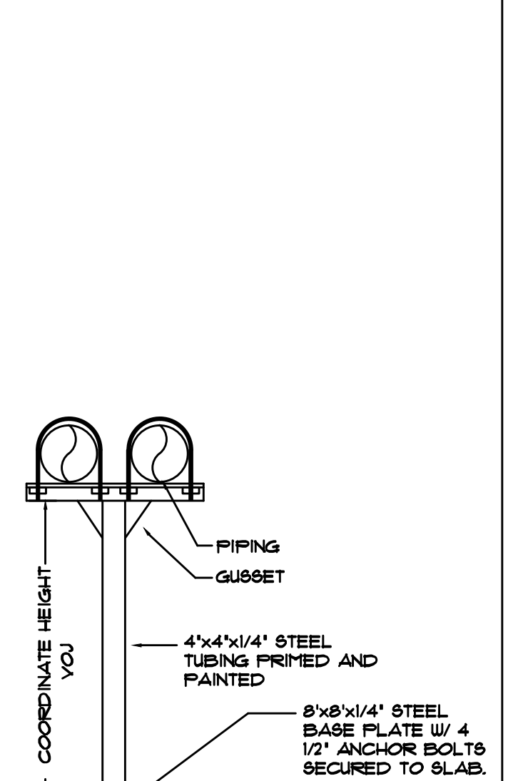
11 PIPE STAND SUPPORT DETAIL M4.3 NO SCALE
