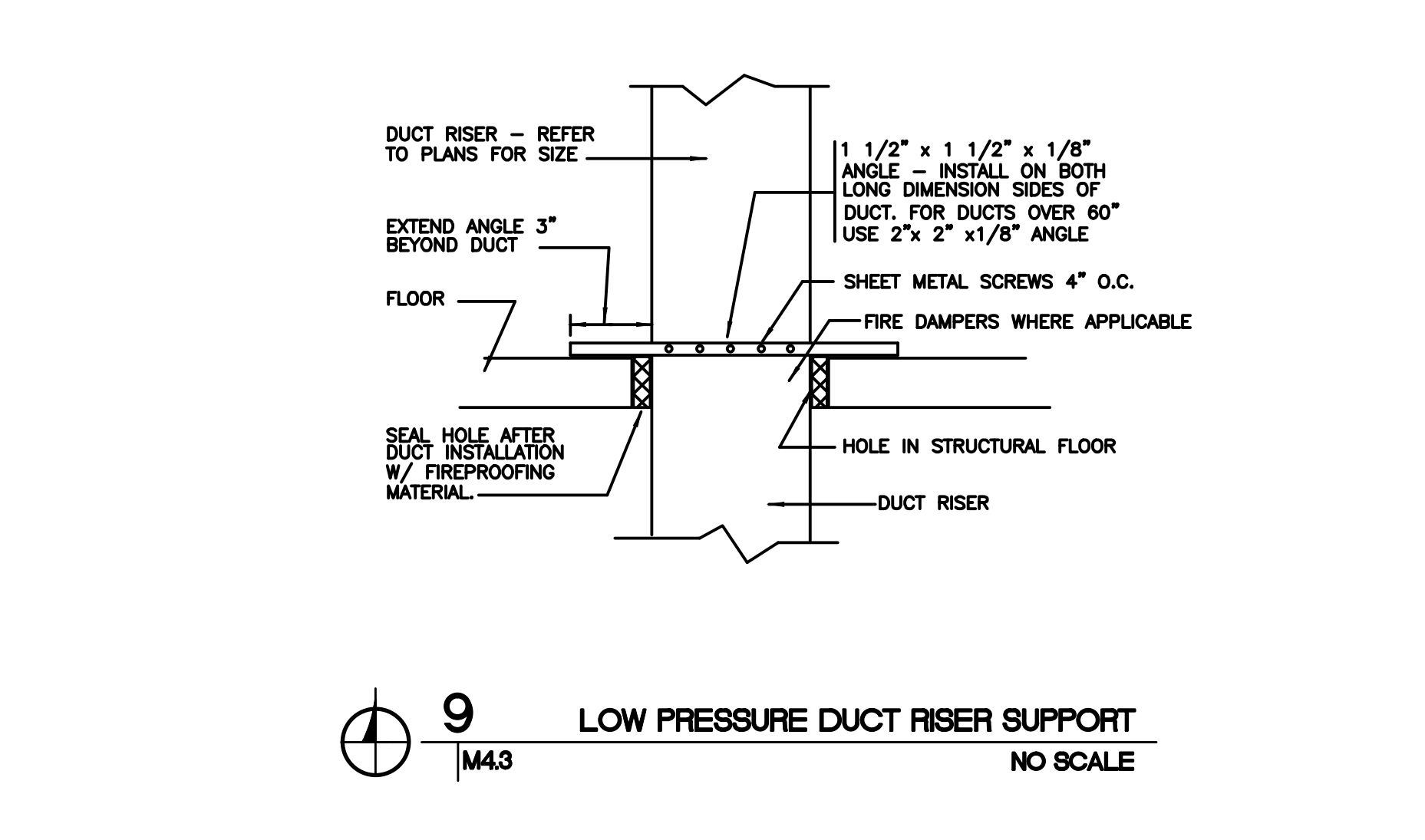
9 LOW PRESSURE DUCT RISER SUPPORT M4.3 NO SCALE
