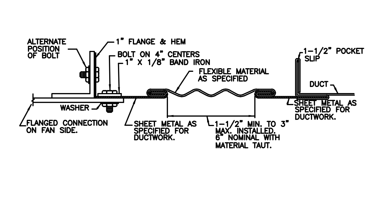
4 RECTANGULAR DUCT FLEX CONNECTION M4.3 NO SCALE
