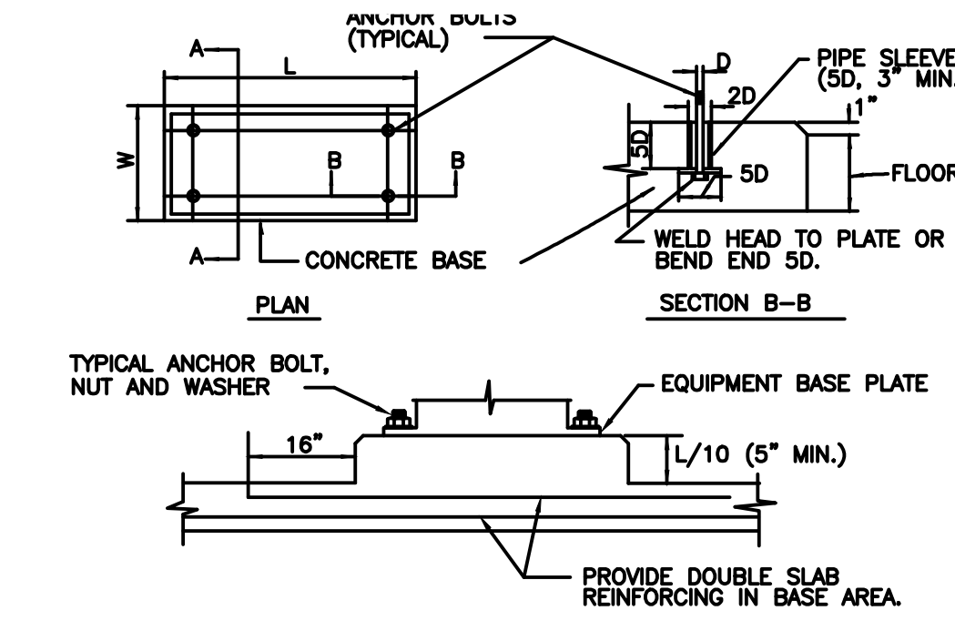
5 CONCRETE EQUIPMENT BASES M4.3 NO SCALE
