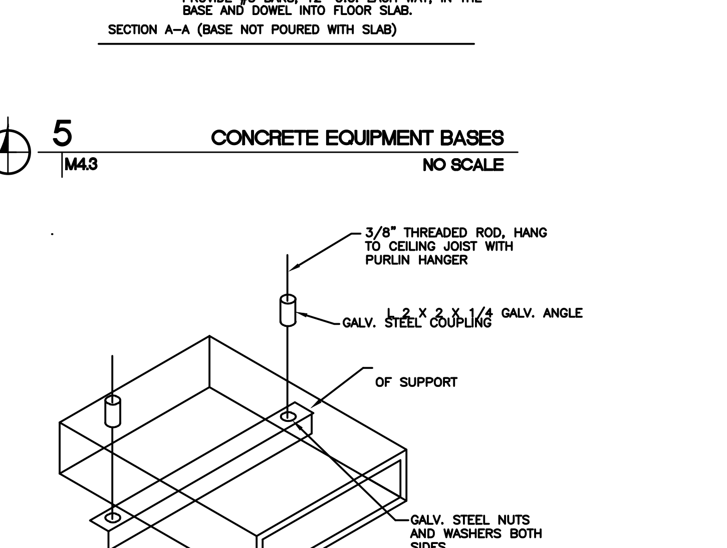
10 DUCT SUPPORT DETAIL (TRAPEZE HANGER) M4.3 NO SCALE
