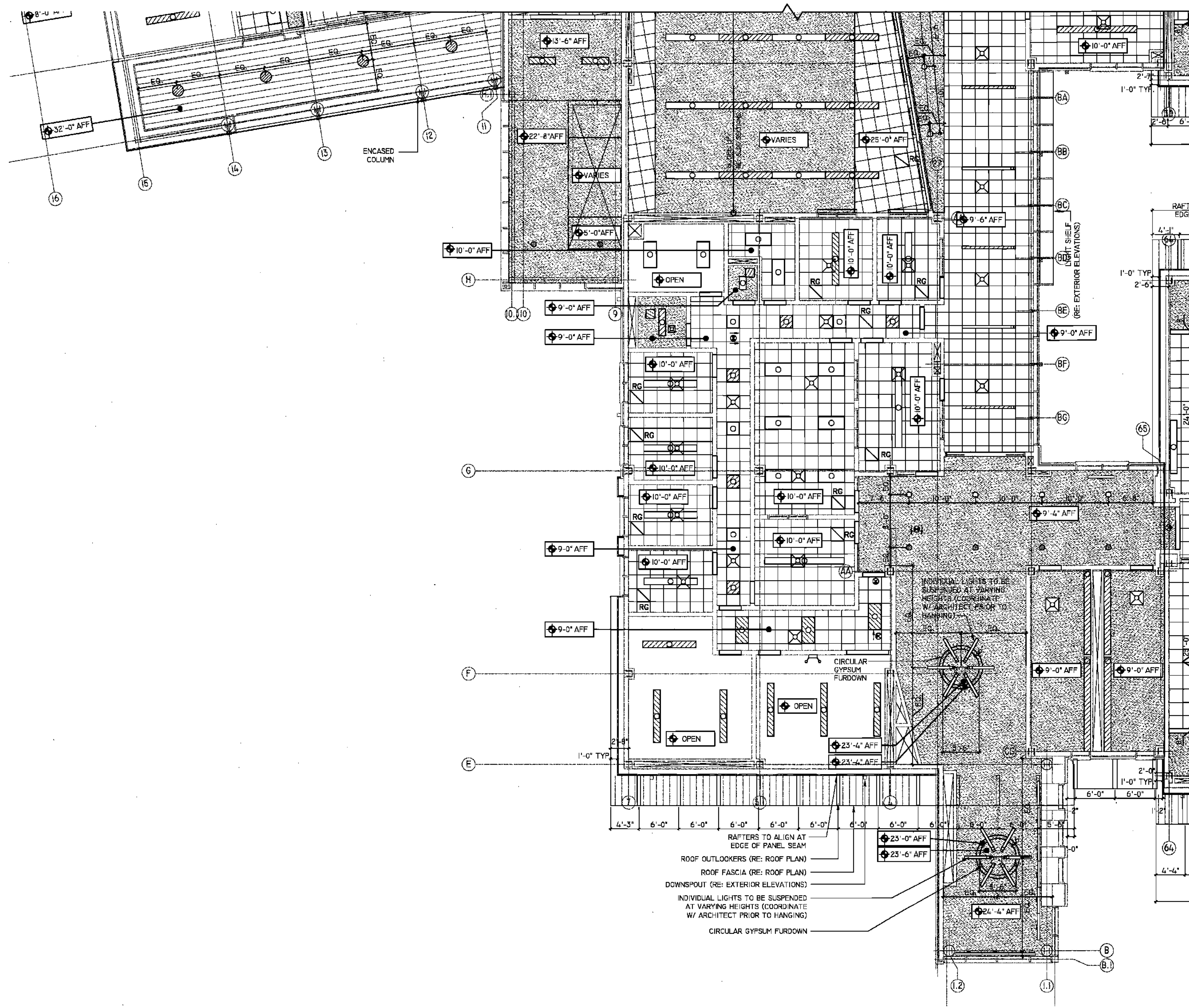
1 PARTIAL SECOND FLOOR REFLECTED CEILING PLAN 1/8" = 1'-0"
