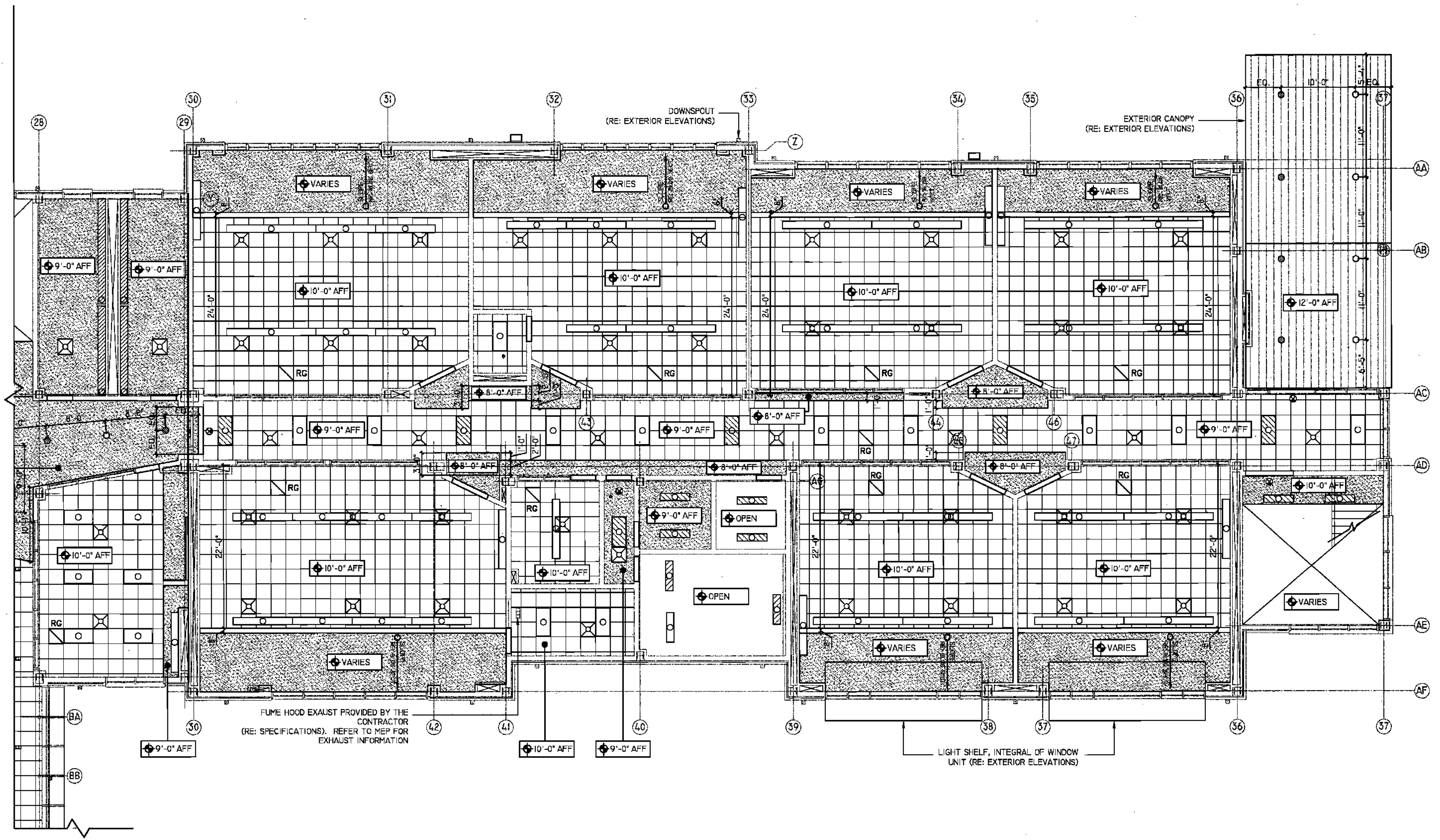
1 PARTIAL FIRST FLOOR REFLECTED CEILING PLAN 1/8" = 1'-0"
