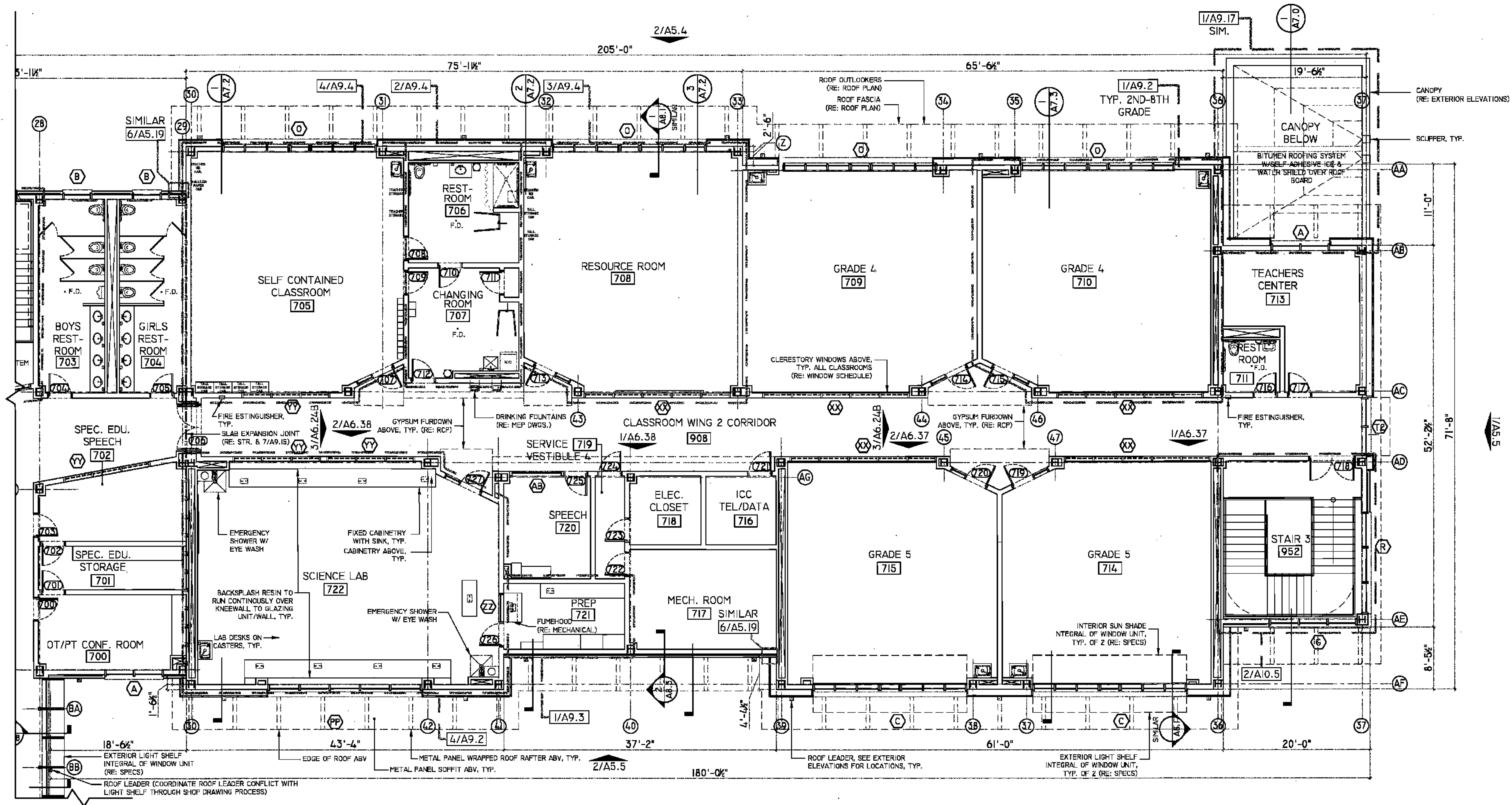
1 SECOND FLOOR PLAN 1/8" = 1'-0"
