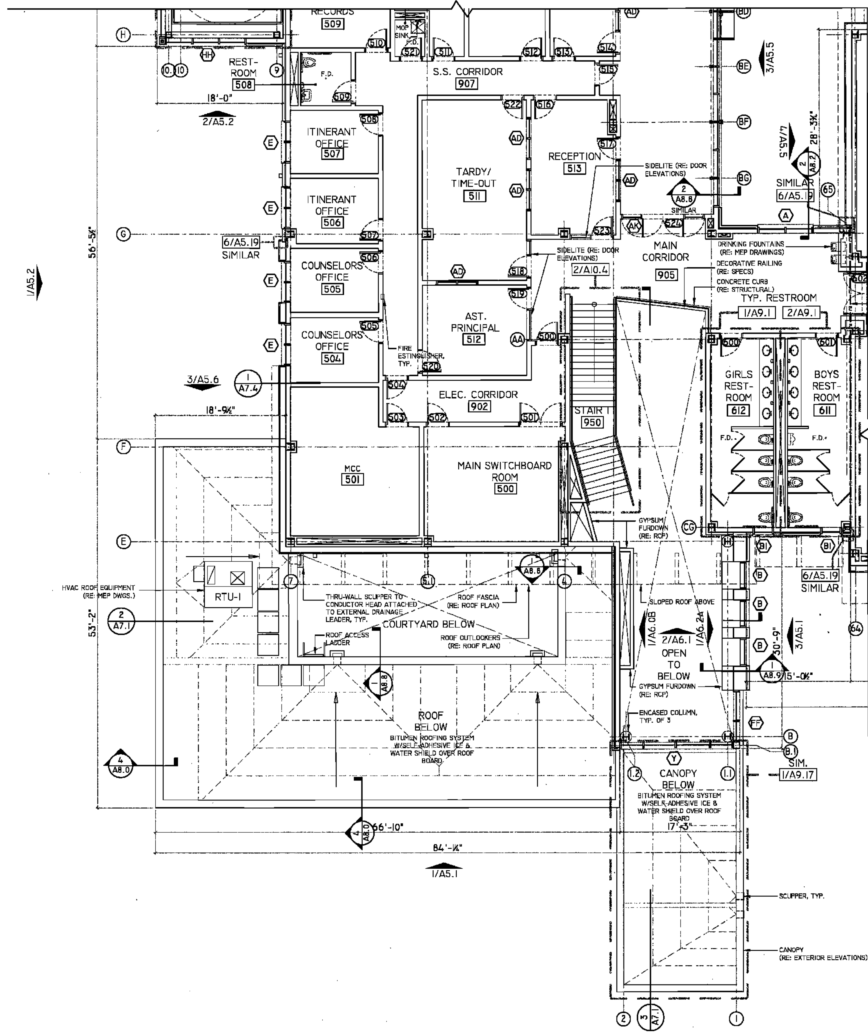
1 SECOND FLOOR PLAN 1/8" = 1'-0"
