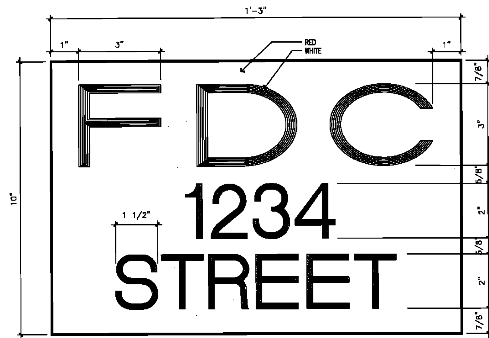
FIRE CONNECTION SIGNAGE CONFIRM ACTUAL LOCATION WITH ARCHITECT PRIOR TO INSTALLATION. SIGNAGE - TYPE 'J'
