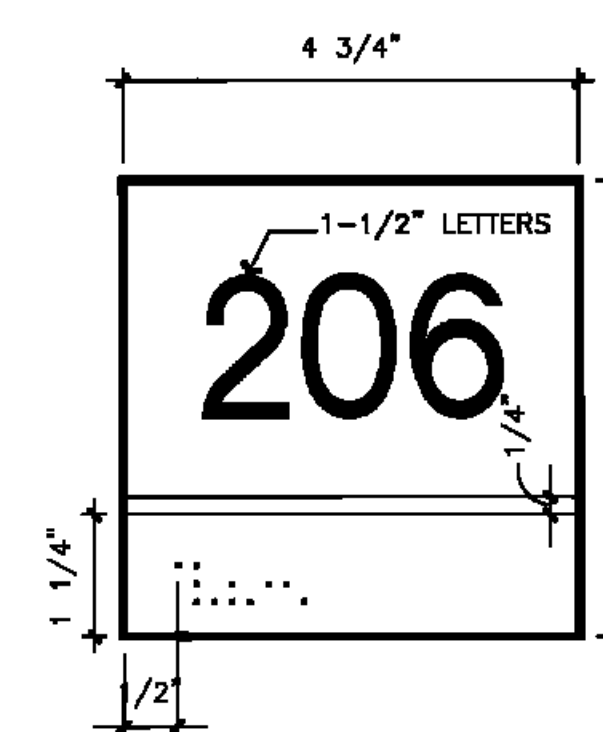
SIGNAGE - TYPE 'D'
