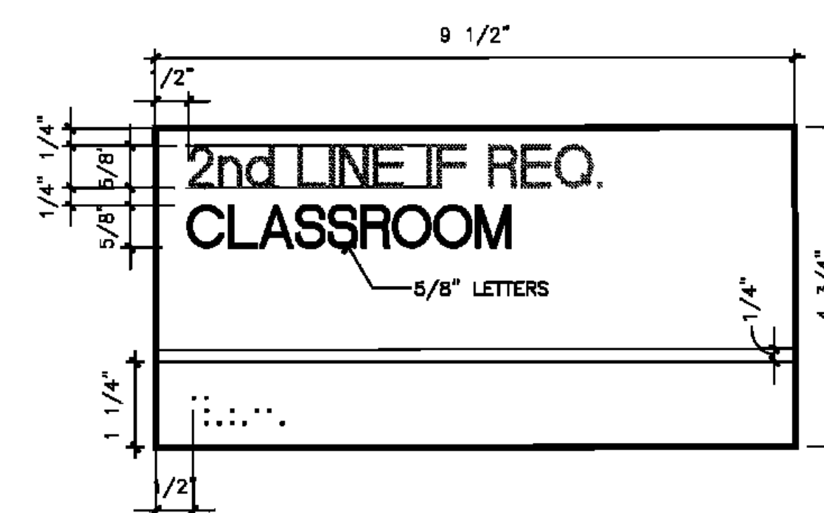
SIGNAGE - TYPE 'C'
