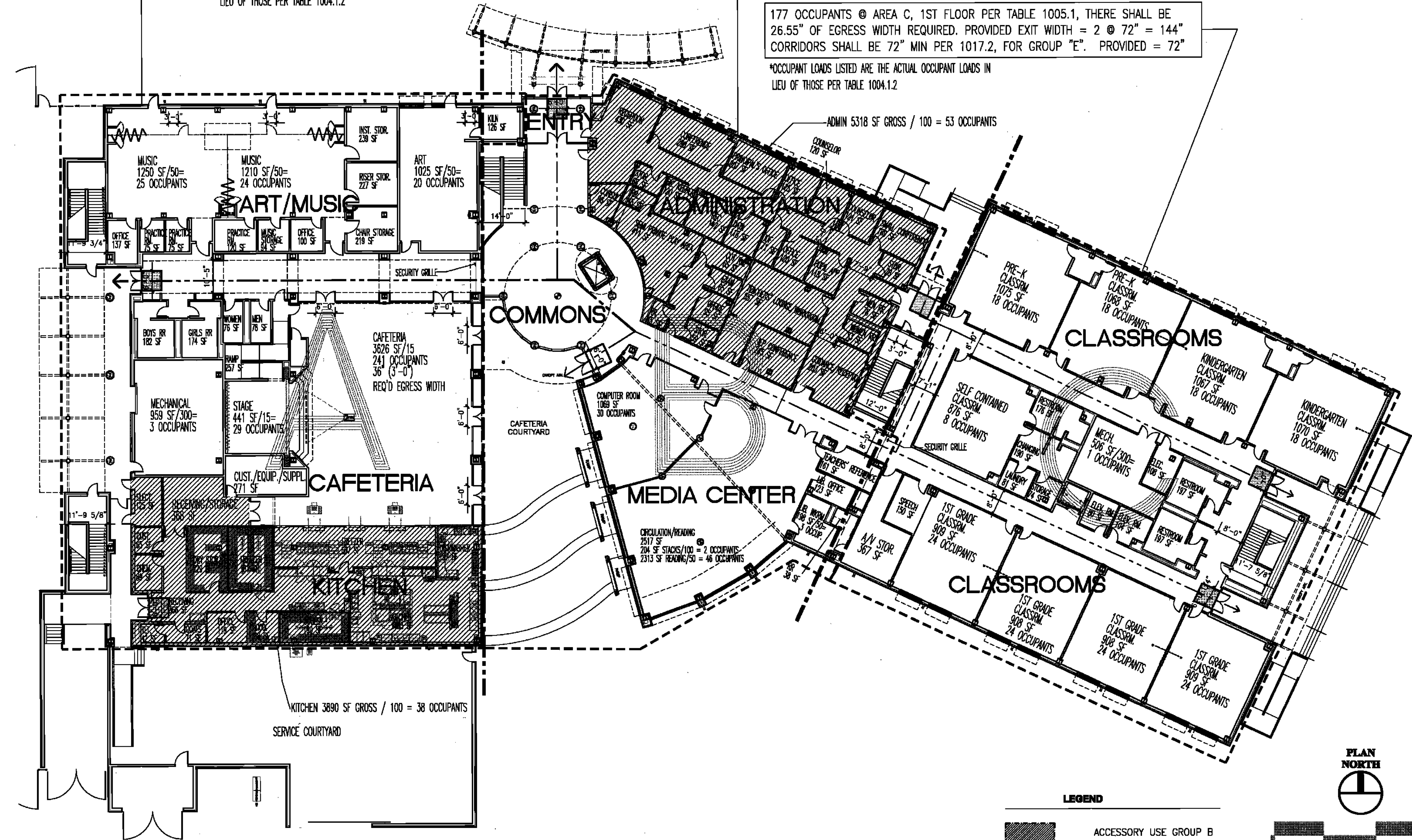
6 FIRST FLOOR EGRESS PLAN
