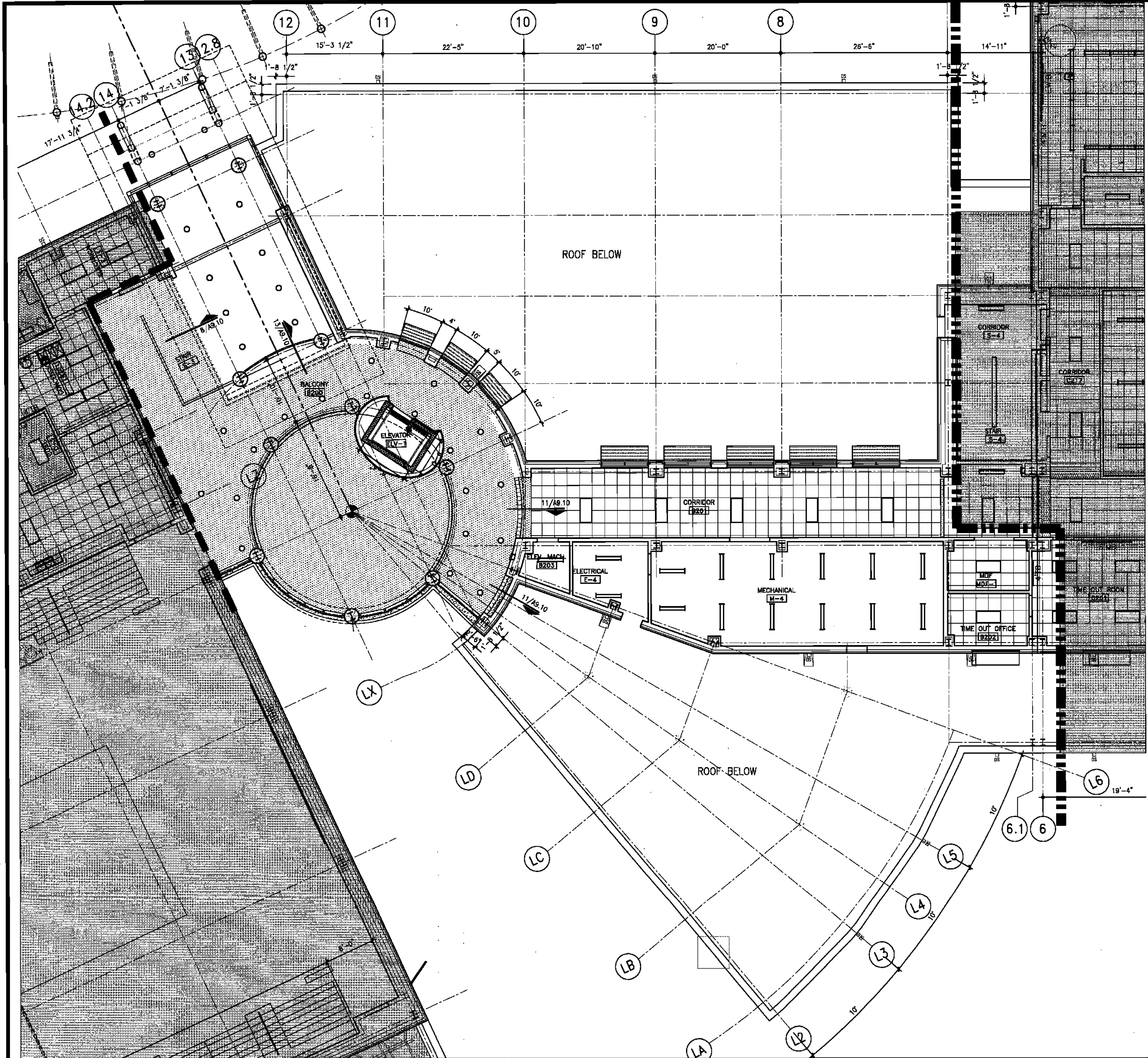
6 REFLECTED CEILING PLAN - SECOND FLOOR - AREA "B"
