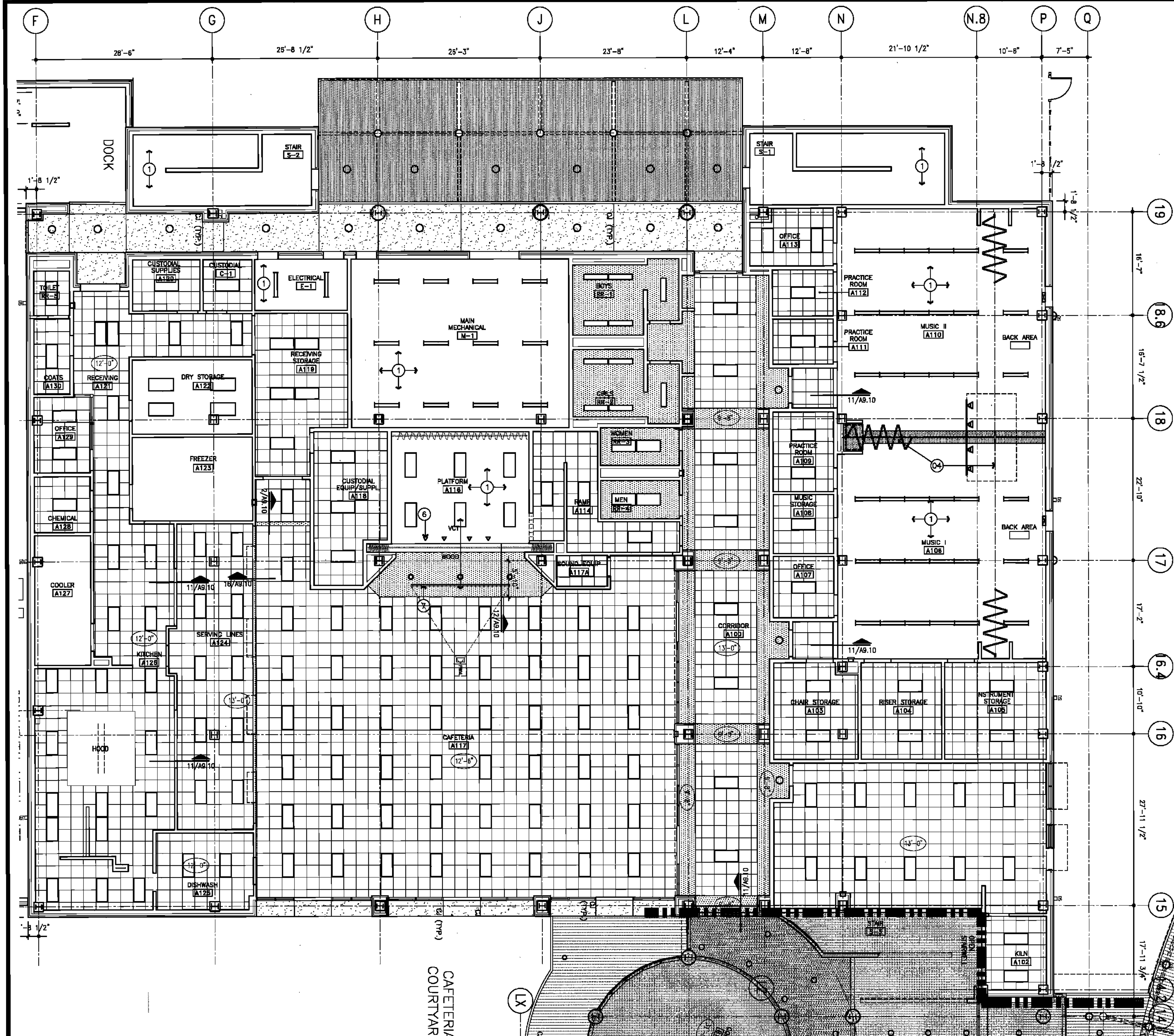
6 REFLECTED CEILING PLAN - FIRST FLOOR - AREA "A"
