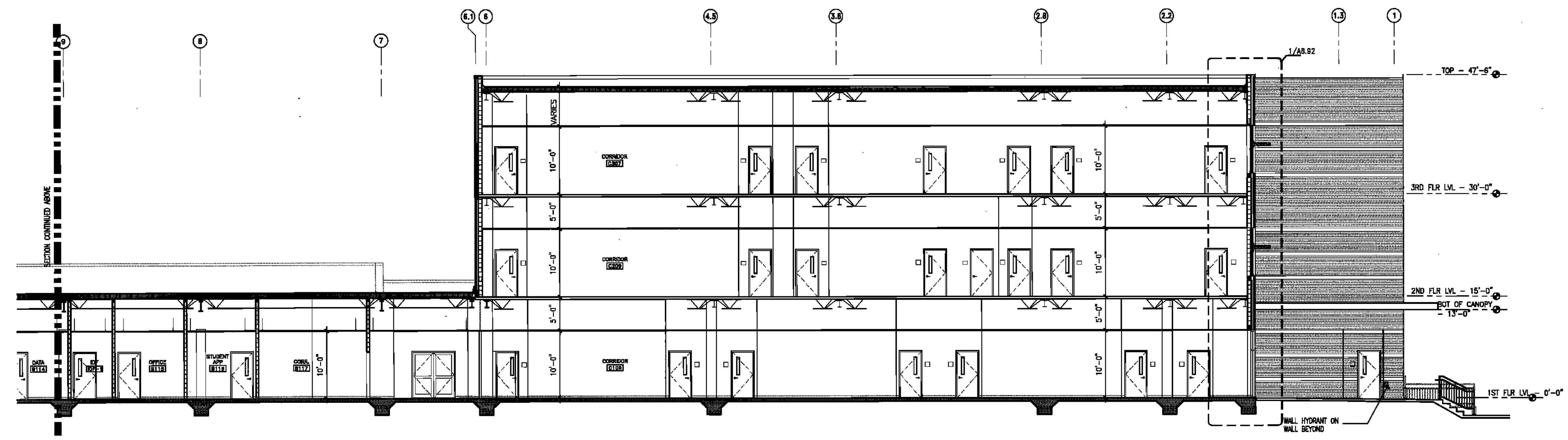
6 BUILDING SECTION - CLASSROOM AND GYMNASIUM WINGS LOOKING NORTH
