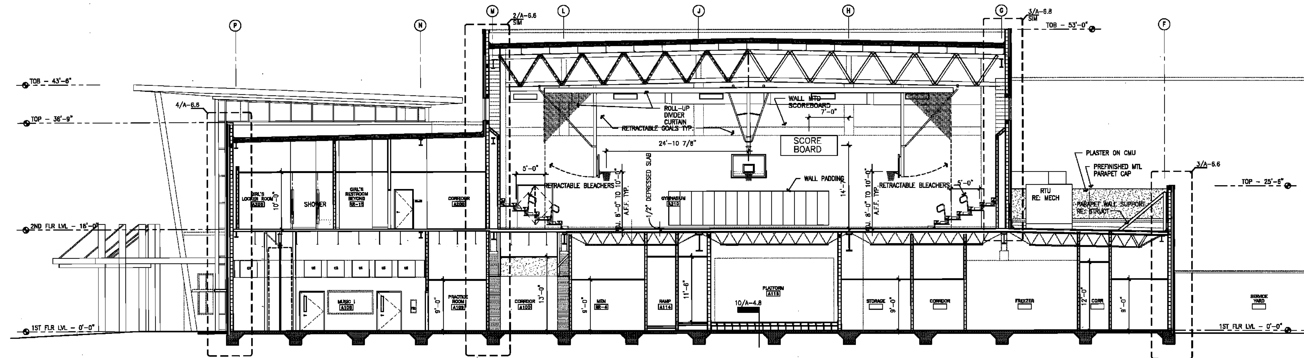
6 BUILDING SECTION THROUGH GYMNASIUM AND MUSIC ROOM LOOKING EAST
