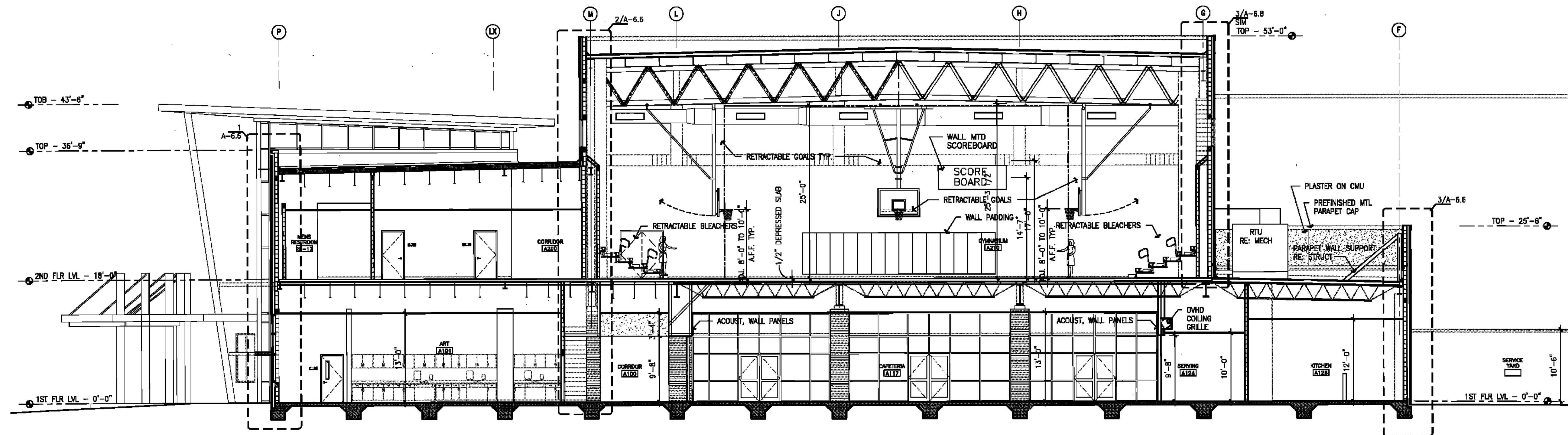
15 BUILDING SECTION THROUGH ART ROOM AND GYMNASIUM LOOKING EAST
