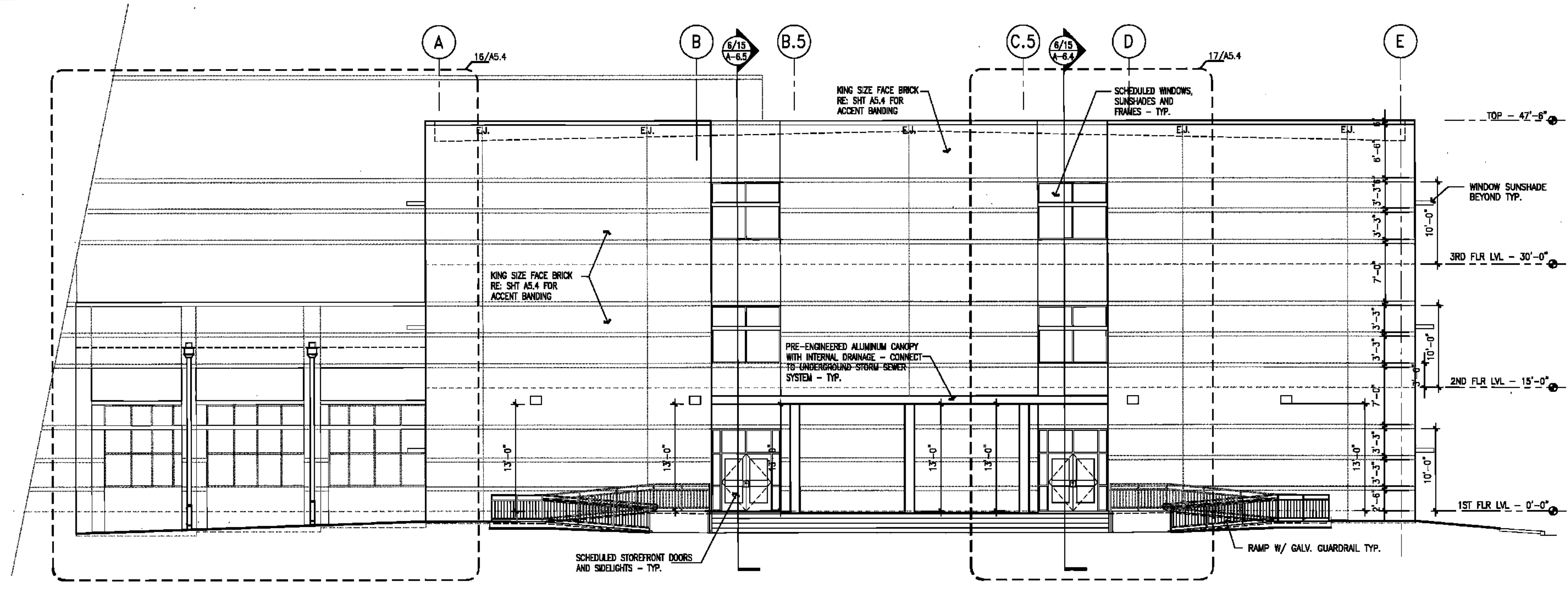
6 BUILDING ELEVATION - THIRD STREET SIDE - AREA C
