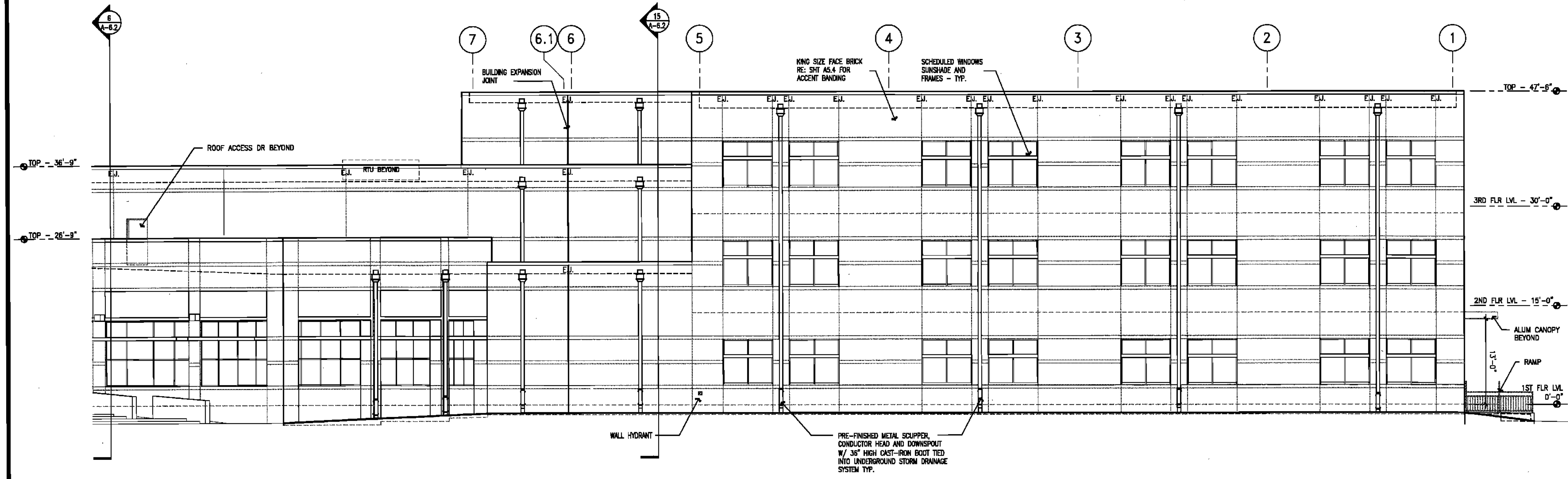
15 BUILDING ELEVATION - PARTIAL FRERET SIDE - AREA C
