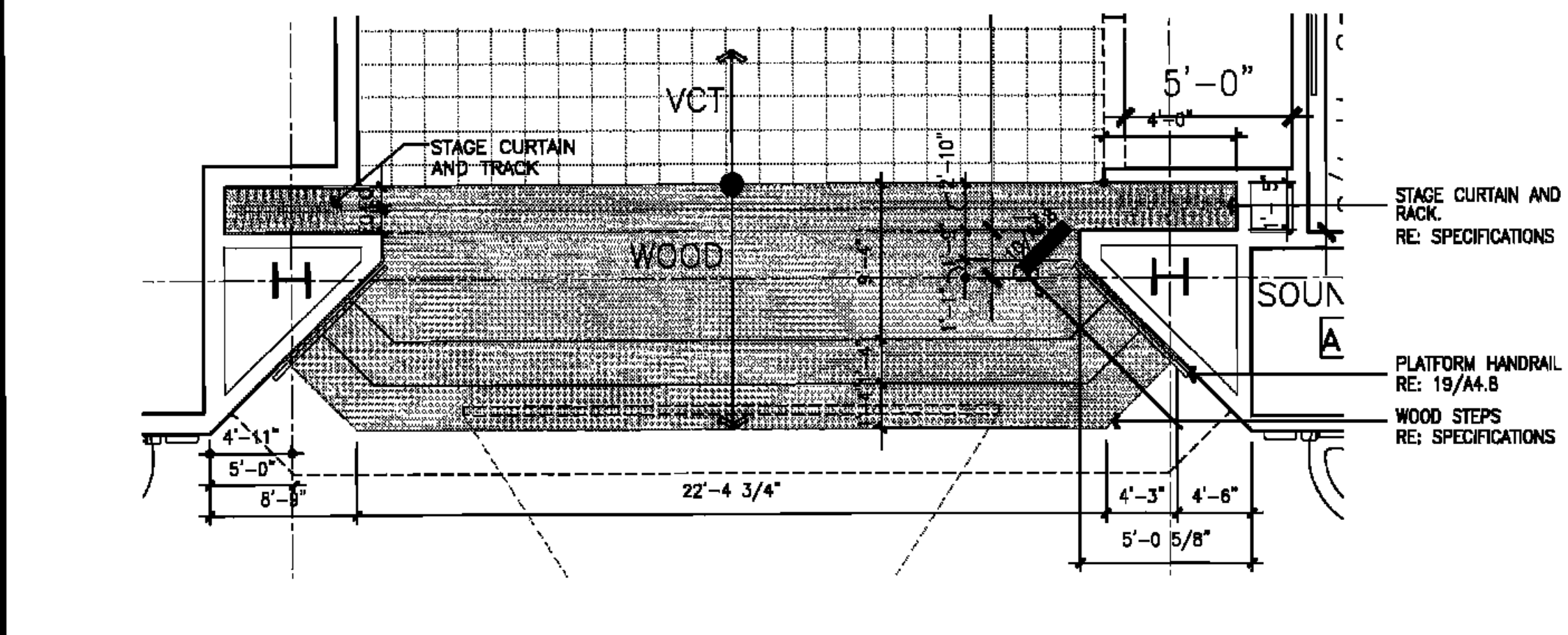
15 ENLARGED PLATFORM PLAN 1/4" = 1'-0"
