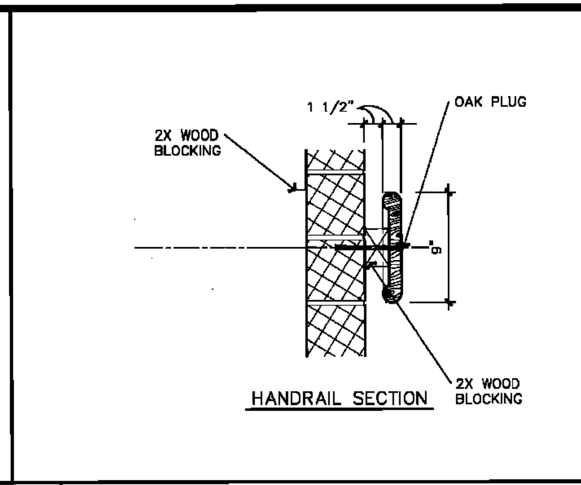
19 STAGE HANDRAIL SECT. 1 1/2" = 1'-0"
