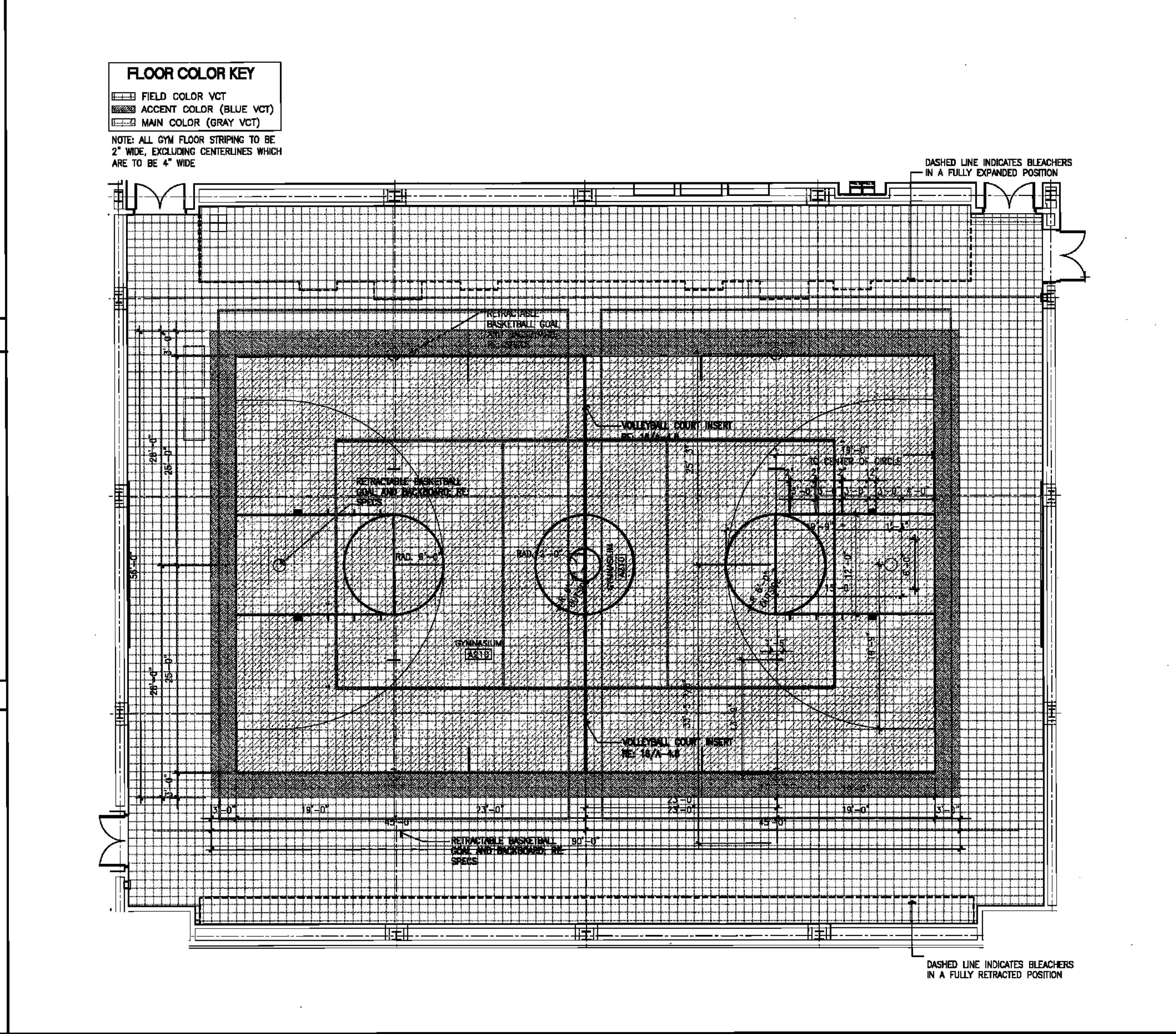
3 ENLARGED COURT STRIPING PLAN 1/8" = 1'-0"
