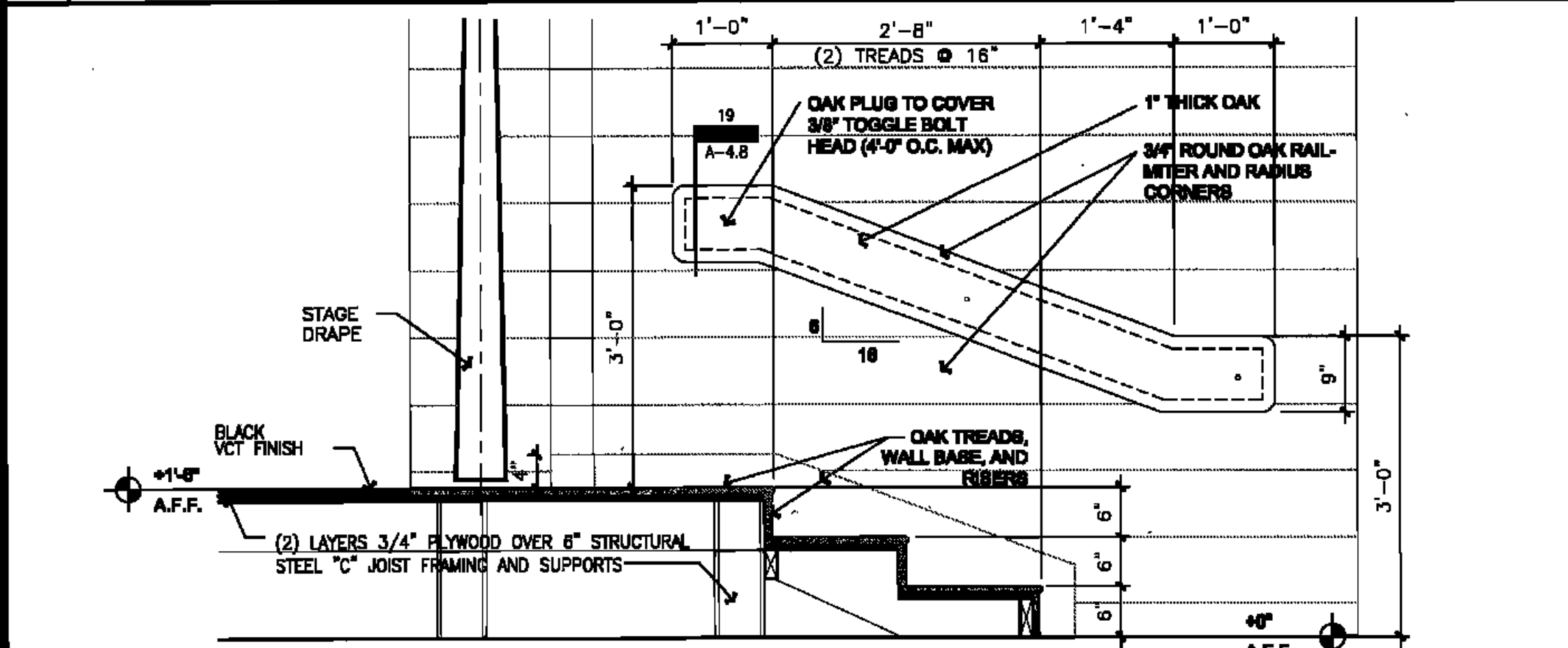
10 STAGE STEP DETAIL STAGE STAIR.dwg 3/4" = 1'-0"
