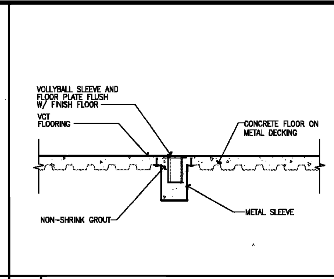
16 VOLLEYBALL INSERT 3/4" = 1'-0"
