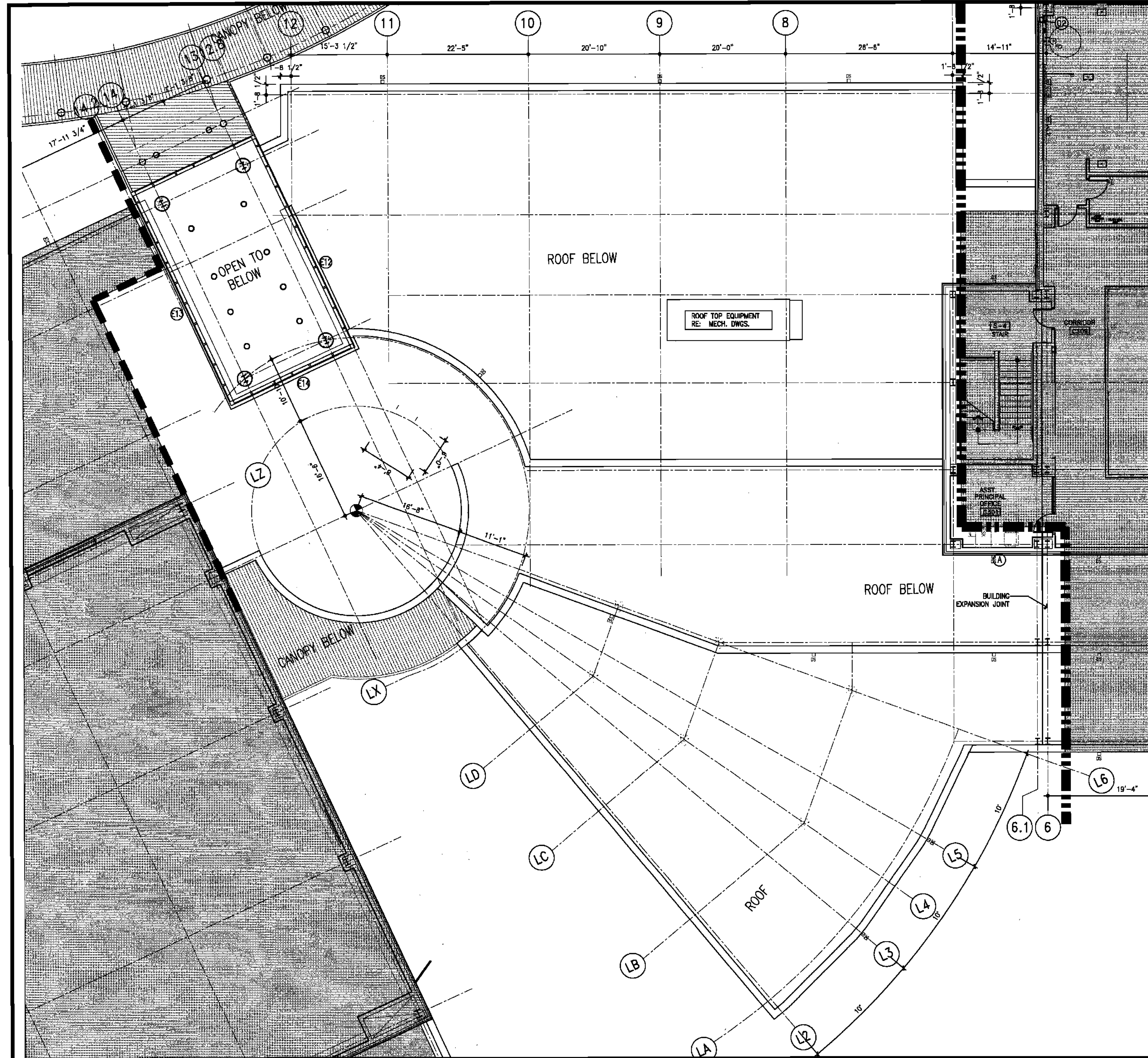
6 THIRD FLOOR PLAN - AREA "B"
