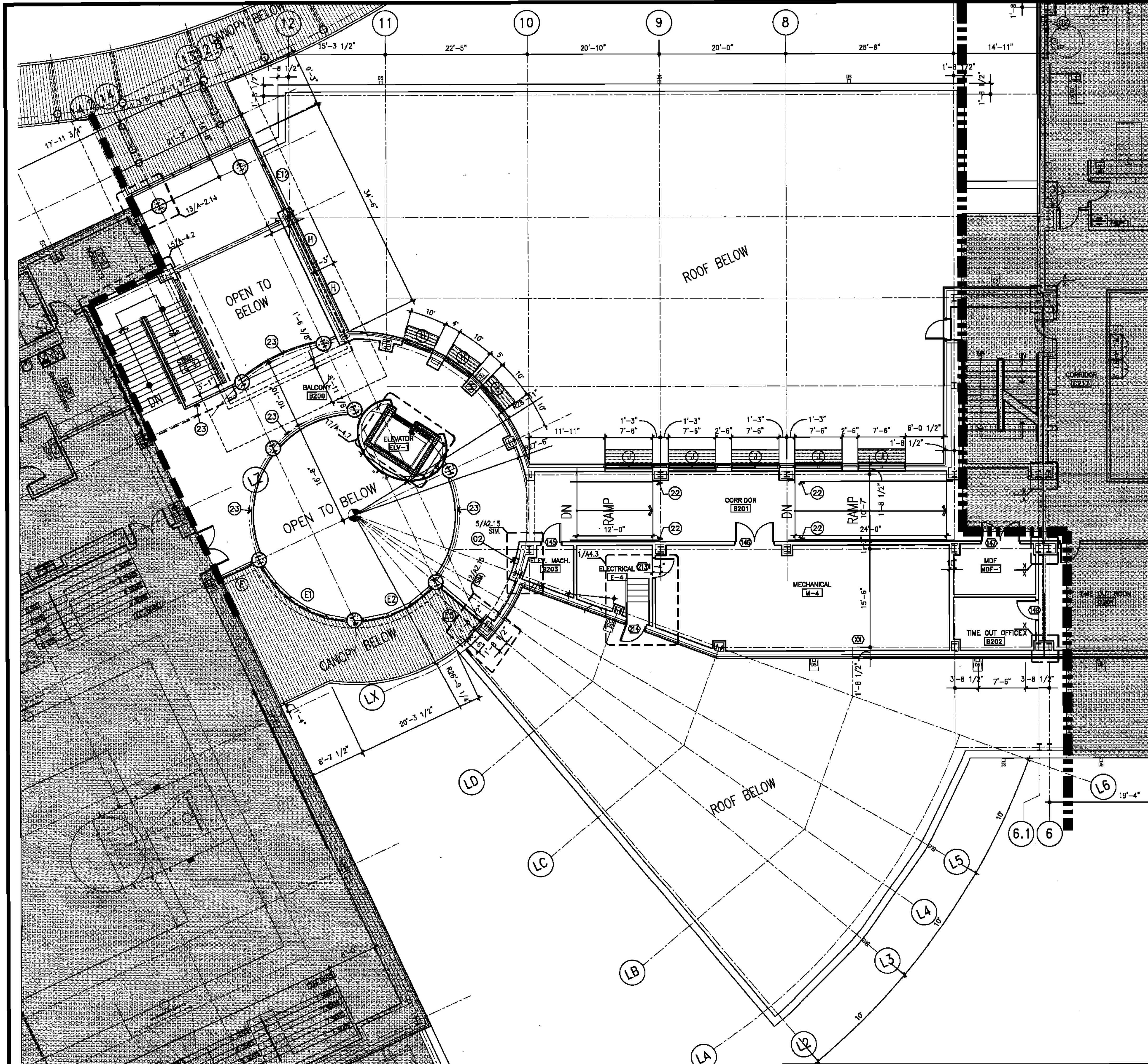
6 SECOND FLOOR PLAN - AREA "B"
