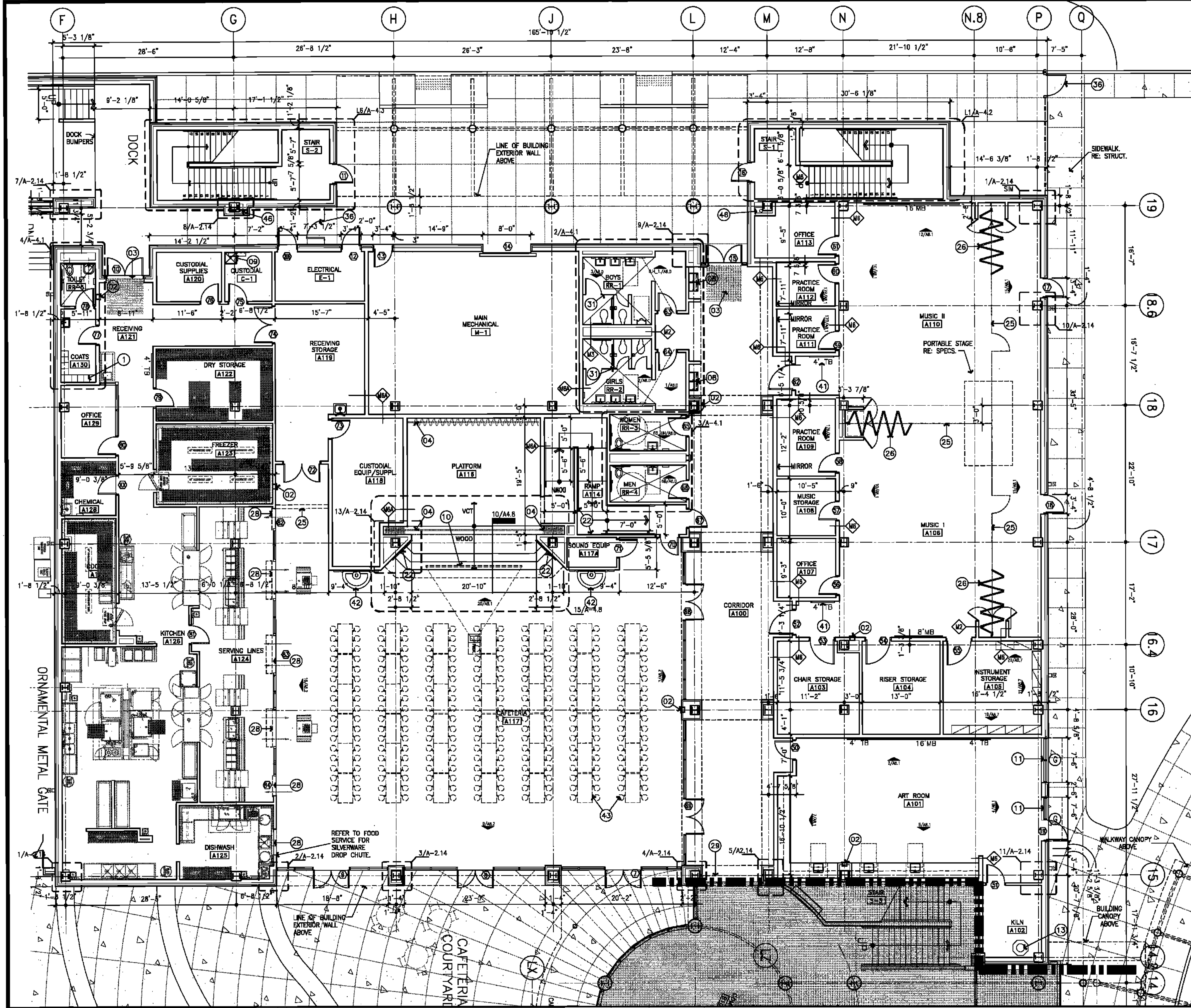
6 FIRST FLOOR PLAN - AREA 'A'
